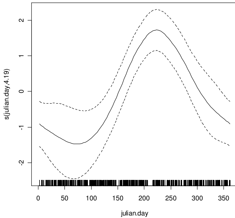
Figure 17: Seasonal pattern in the number of sightings of harbour porpoise within the study area (animals observed hour -1 ).
